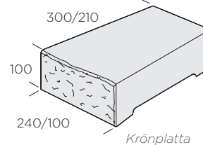
Krönplatta
